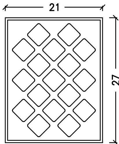
17 Lites 21" x 27"
