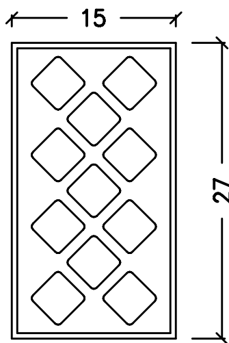
11 Lites 15" x 27"
