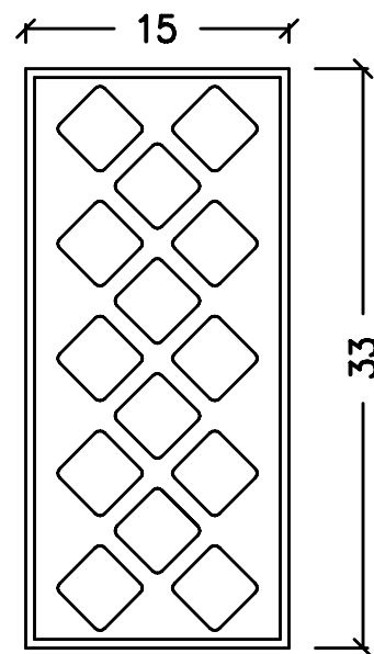
14 Lites 15" x 33"
