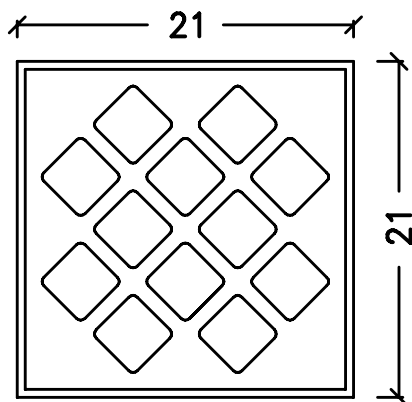
12 Lites 21" x 21"
